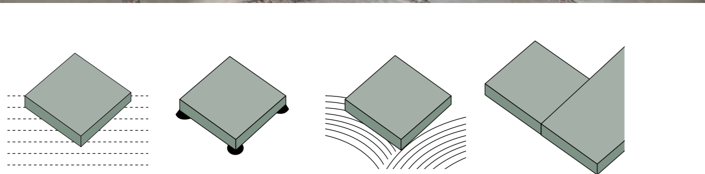
DRY INSTALLATION ON GRAVEL, GRASS OR SAND
