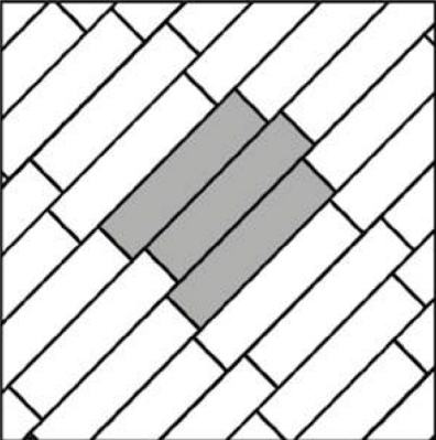
Staggered Laying ( Max 15% - % 20 )
